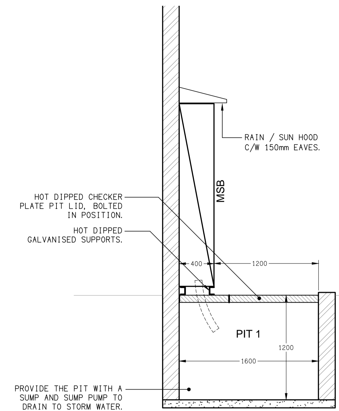
DETAIL A MSB & PIT 1 SECTION NOT TO SCALE
